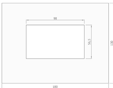
FRAME DISPLAY (VALID FOR STEEL AND WOOD VERSION)
